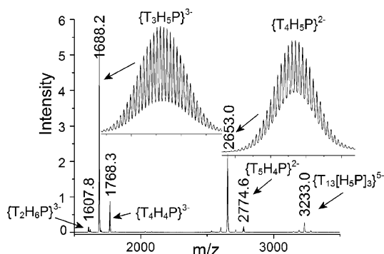
Figure 3. The negative ion mass spectrum of the TBA + salt of 2 showing the series of tetra-, penta-, and hexaprotonated forms of (TBA) n [H 5 P 1 W 18 O 62 ] 11-(x+y)- in solution. T ≡ TBA + , P ≡ P 1 W 18 O 62 (intensity × 10 4 ).
