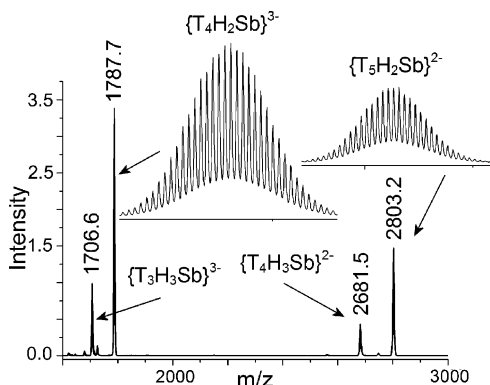
Figure 2. The negative ion mass spectrum of the TBA + salt of 1 showing the series of tri- and tetraprotonated forms of (TBA) n [H 2 SbW 18 O 60 ] 9-(x+y)- in solution. T ≡ TBA + , Sb ≡ Sb 1 W 18 O 60 (intensity × 10 4 ).
